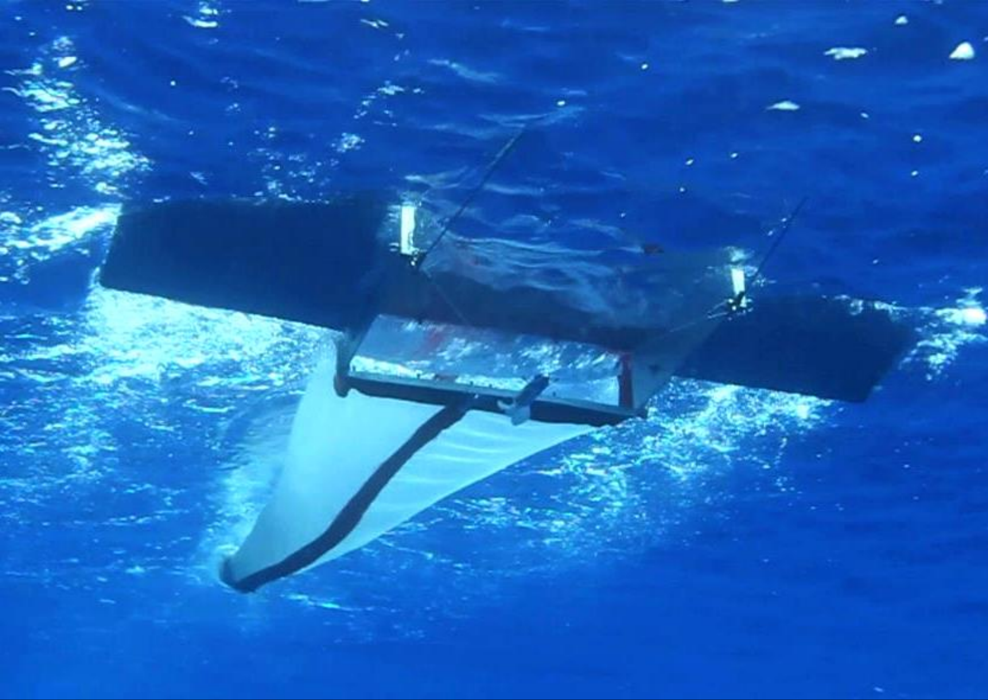
The Manta Trawl
